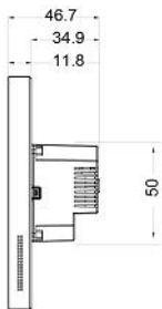
2 RIGHT VIEW
