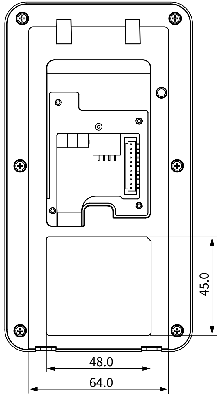
4 BACK VIEW
