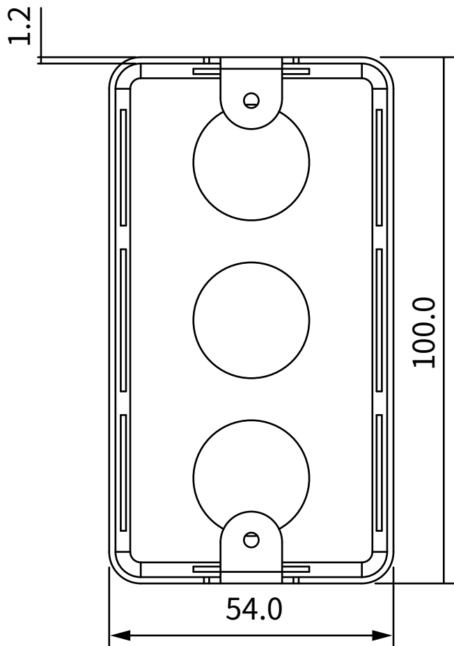
1 FRONT VIEW
