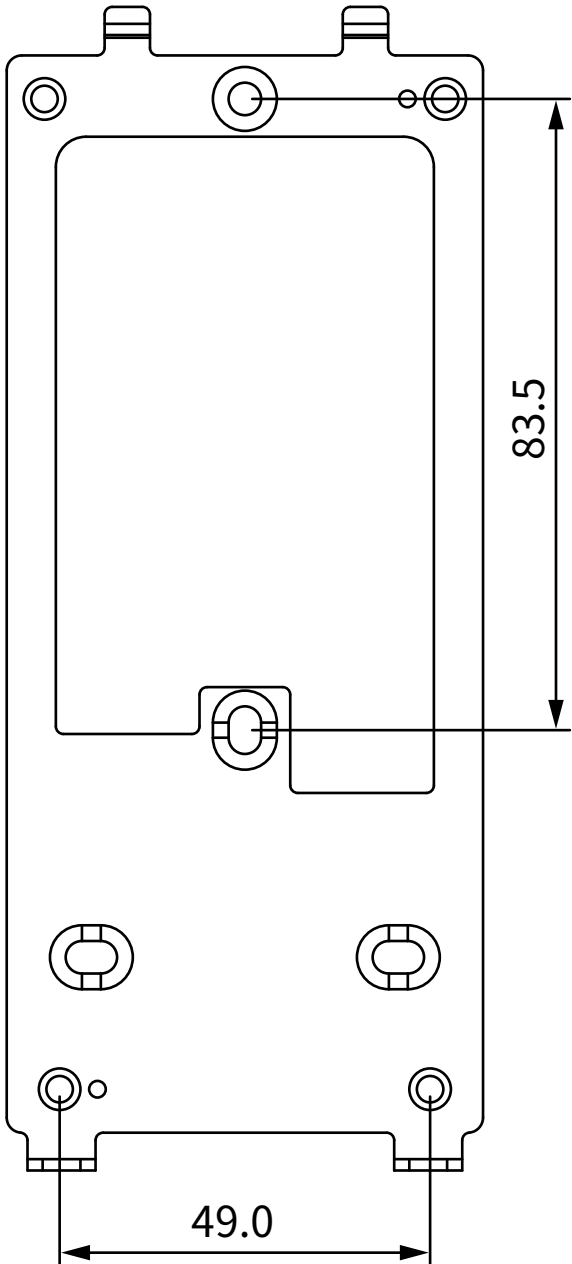
4 BACK VIEW
