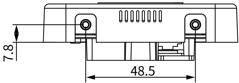
6 BOTTOM VIEW
