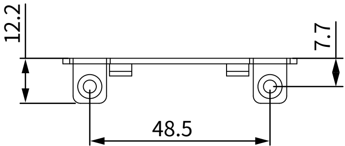
5 TOP VIEW
