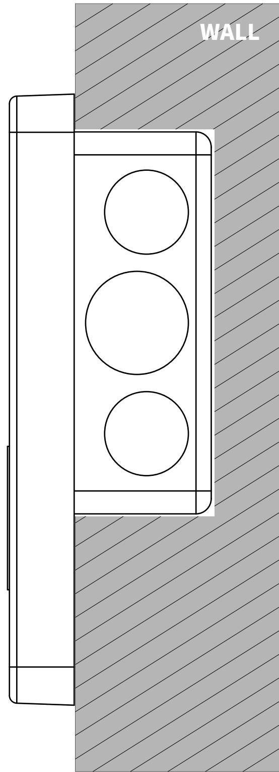
4 SIDE VIEW:INTERCOM PANEL IN WALL
