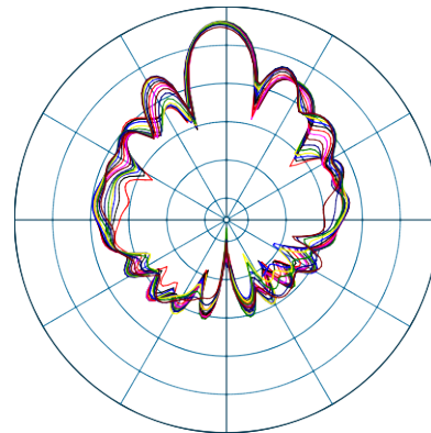
Vertical Elevation
